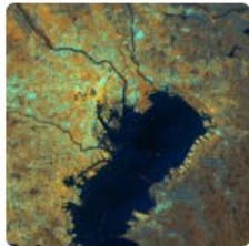
Sentinel-1
