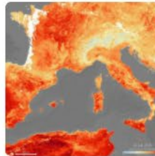
Sentinel-3
