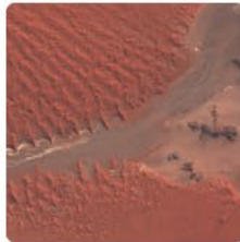
Sentinel-2
